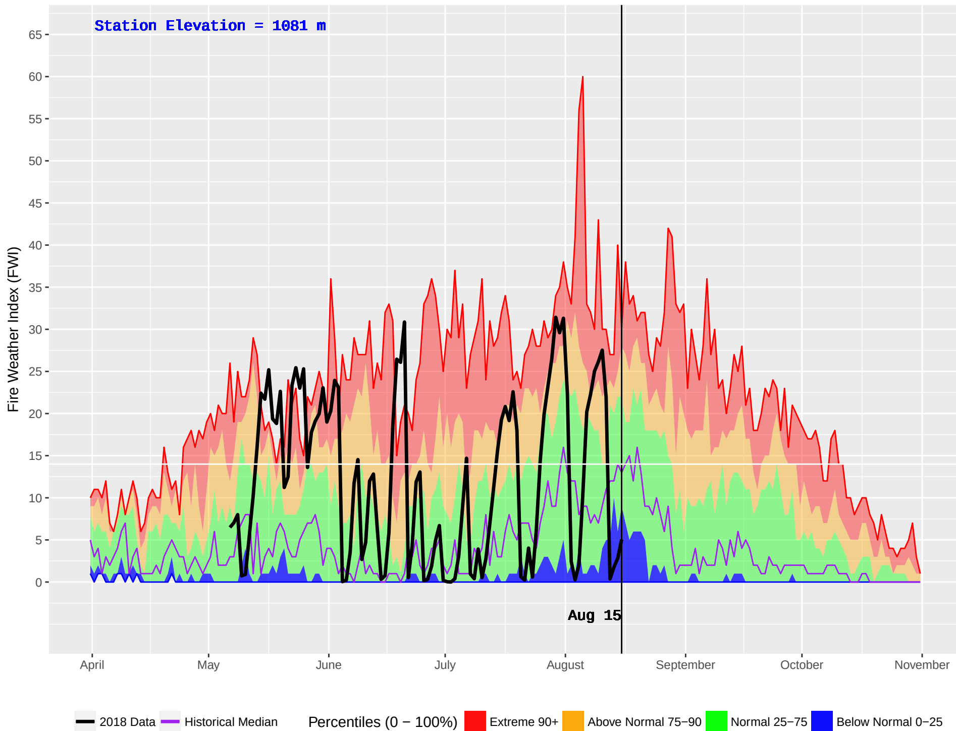
GAVIN (227) : Historical (1981–2016) and Current (2018) Daily Fire Weather Index (FWI)
