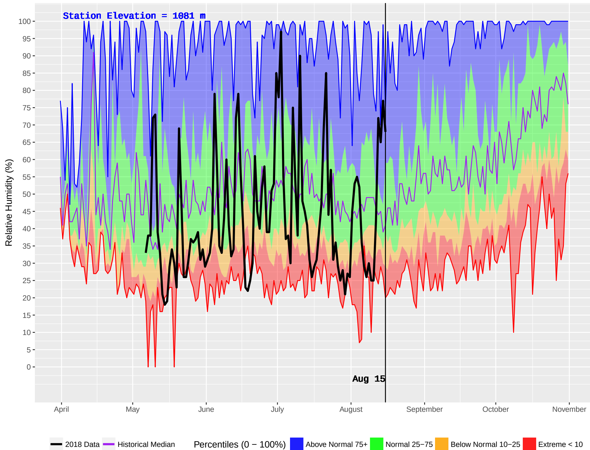
GAVIN (227) : Historical (1981–2016) and Current (2018) Daily Relative Humidity
