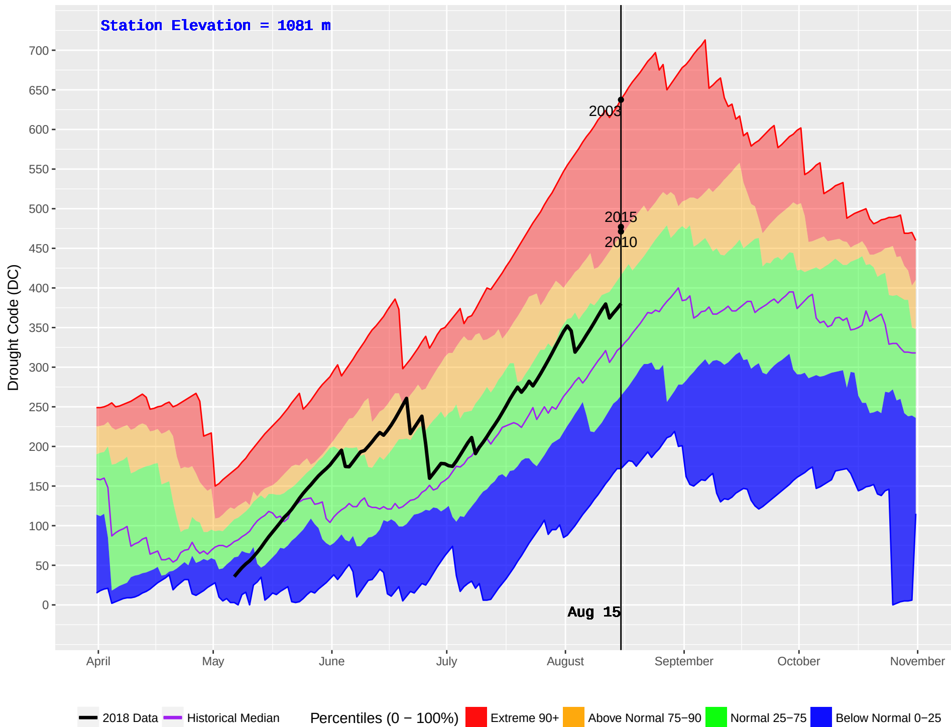
GAVIN (227) : Historical (1981–2016) and Current (2018) Daily Drought Code (DC)
