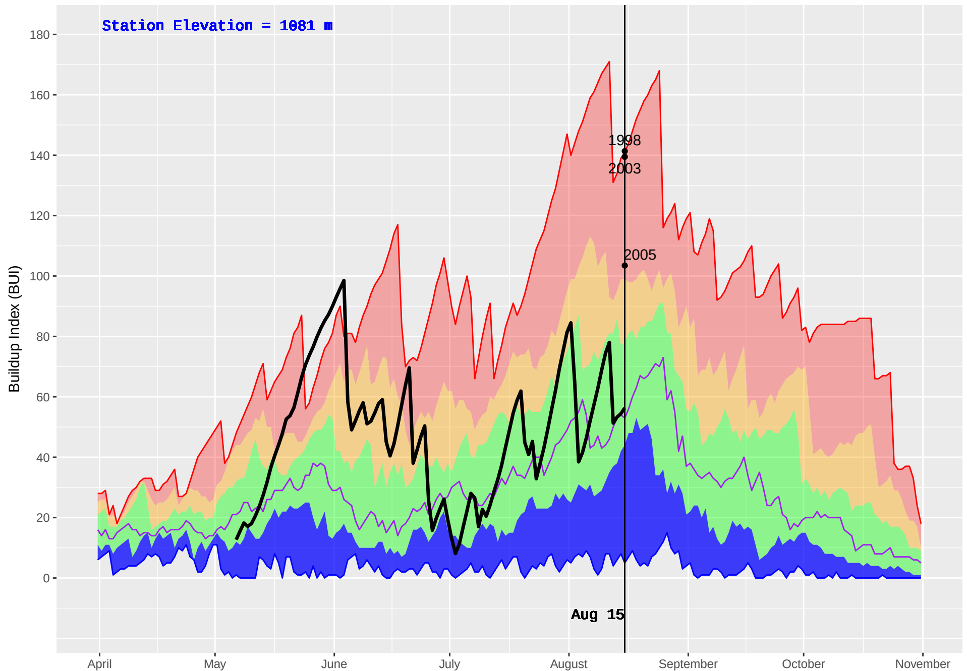
GAVIN (227) : Historical (1981–2016) and Current (2018) Daily Buildup Index (BUI)
