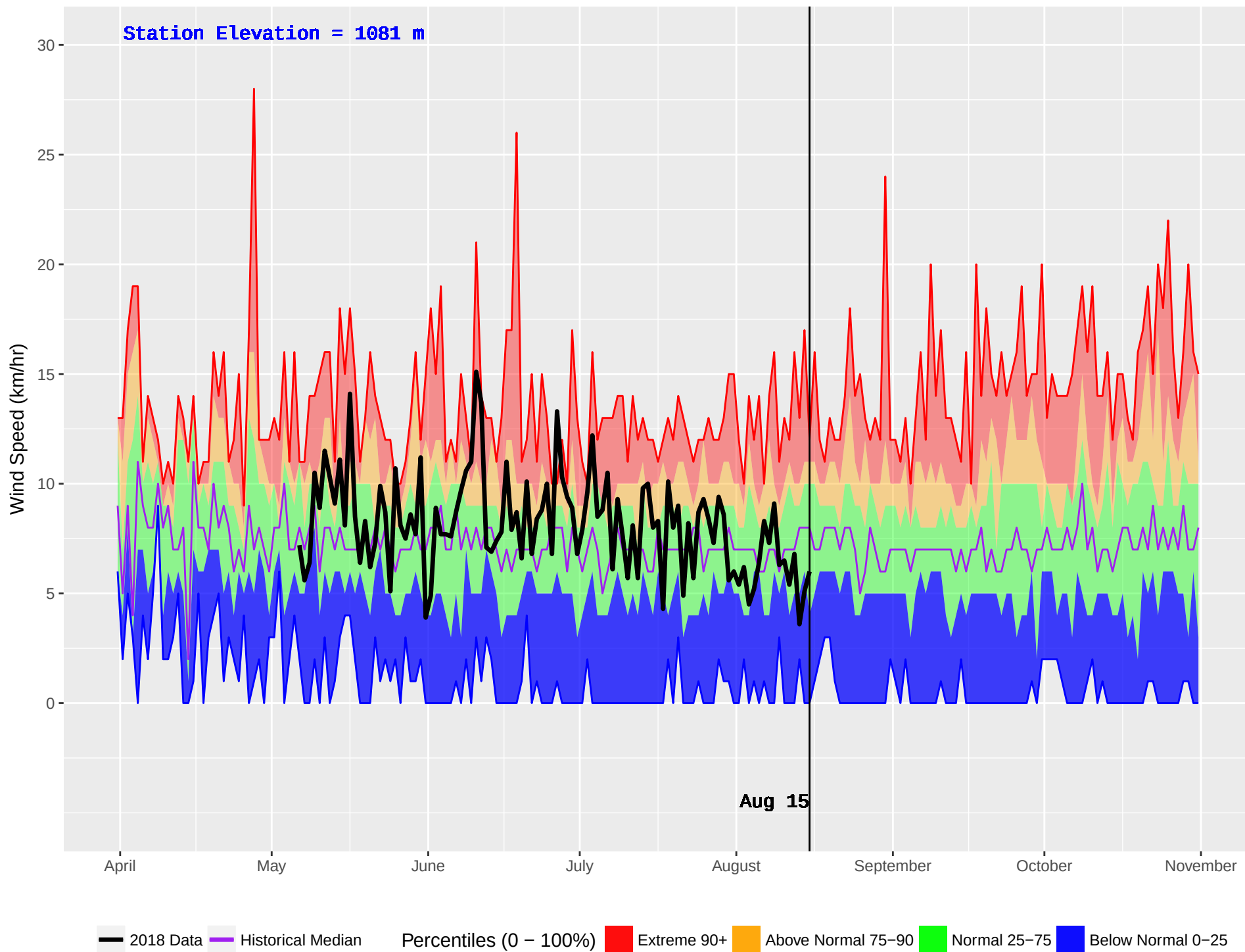
GAVIN (227) : Historical (1981–2016) and Current (2018) Daily Wind Speed
