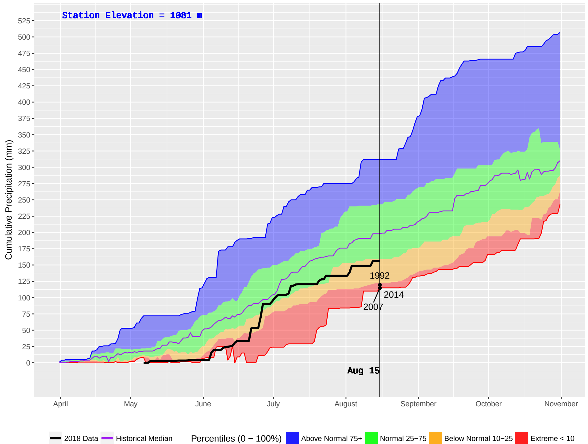
GAVIN (227) : Historical (1981–2016) and Current (2018) Daily Cumulative Precipitation
