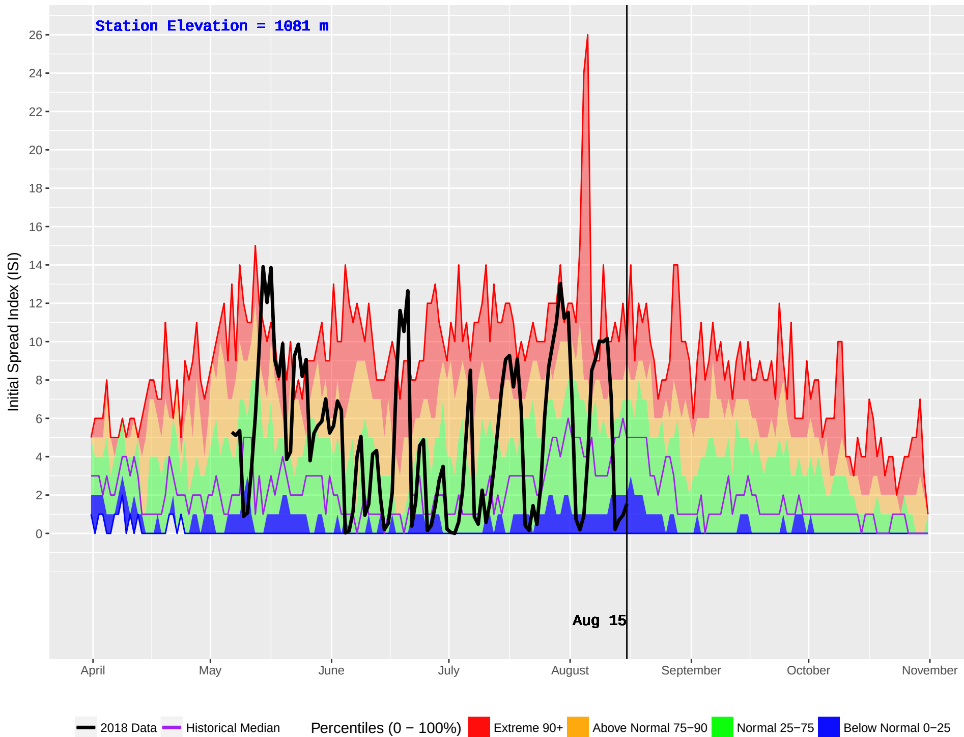
GAVIN (227) : Historical (1981–2016) and Current (2018) Daily Initial Spread Index (ISI)
