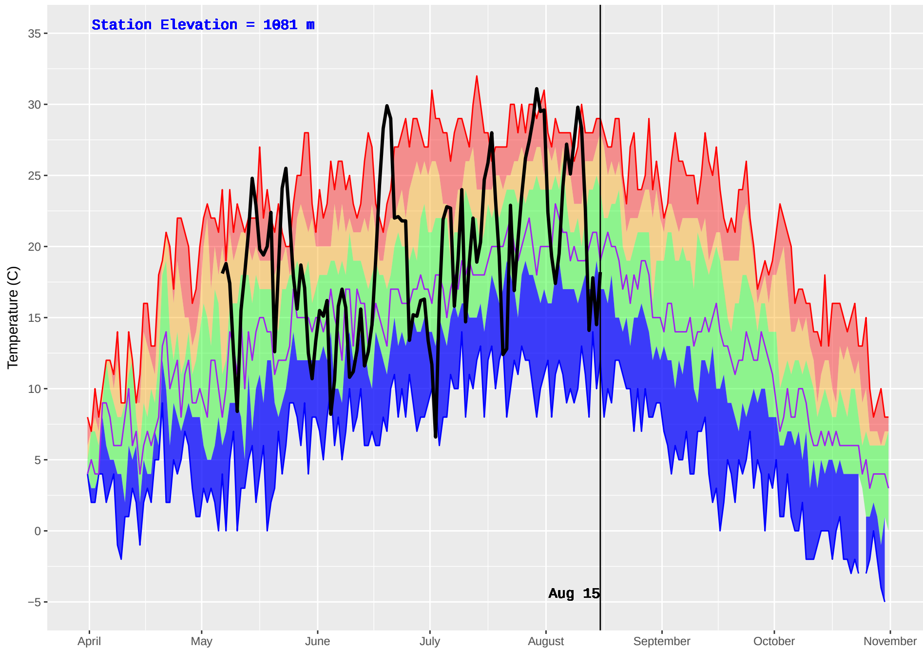
GAVIN (227) : Historical (1981–2016) and Current (2018) Daily Temperature
